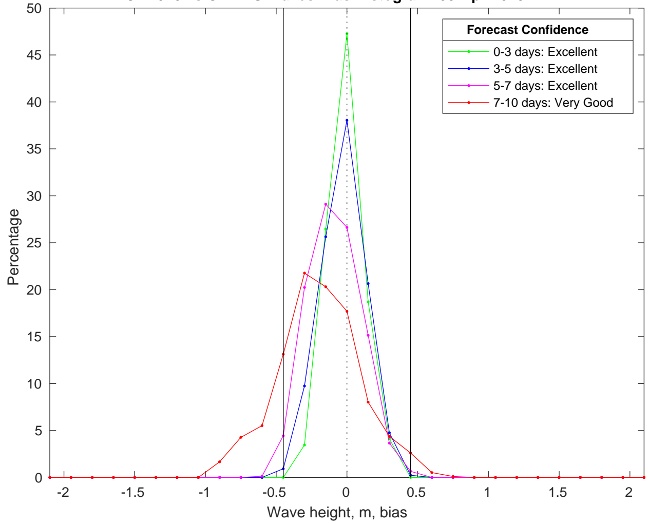
NDBC 41040 vs CMEMS Waves Bias Histogram: 08-Apr-2025
