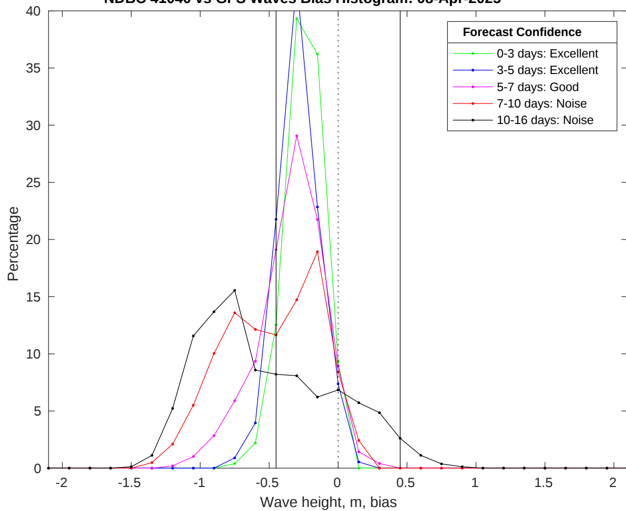
NDBC 41040 vs GFS Waves Bias Histogram: 08-Apr-2025
