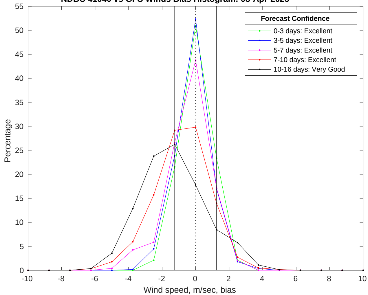
NDBC 41040 vs GFS Winds Bias Histogram: 08-Apr-2025
