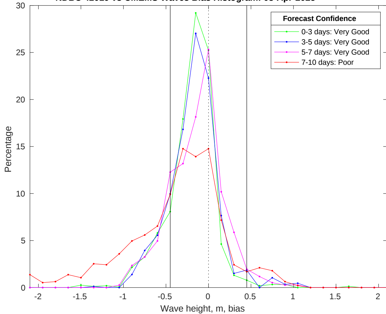
NDBC 42019 vs CMEMS Waves Bias Histogram: 08-Apr-2025
