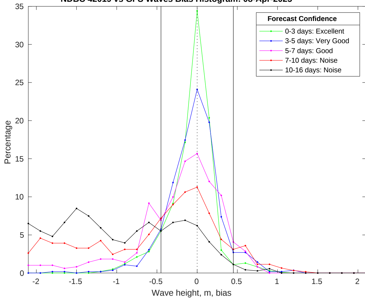
NDBC 42019 vs GFS Waves Bias Histogram: 08-Apr-2025
