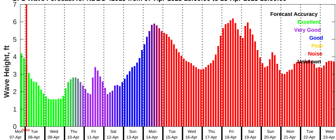
GFS Wave Forecast for NDBC 42019 from 07-Apr-2025 18:00:00 to 23-Apr-2025 18:00:00
