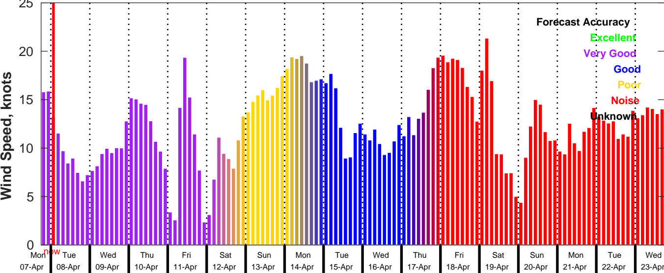
GFS Wind Speed Forecast for NDBC 42019 from 07-Apr-2025 18:00:00 to 23-Apr-2025 18:00:00
