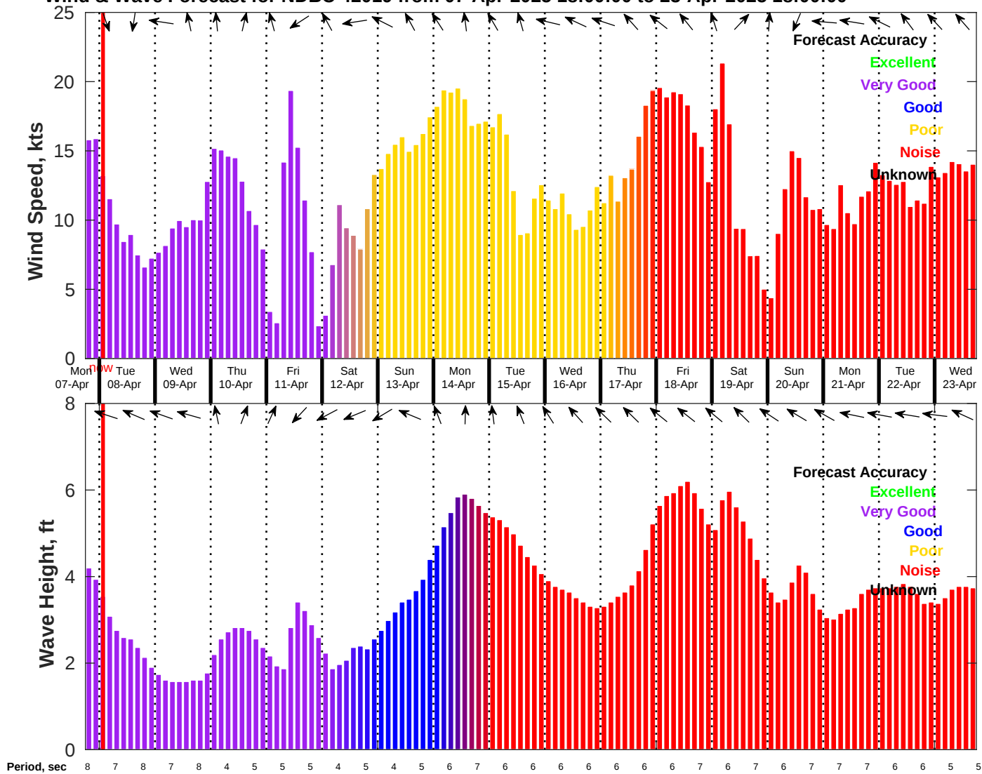
Wind & Wave Forecast for NDBC 42019 from 07-Apr-2025 18:00:00 to 23-Apr-2025 18:00:00
