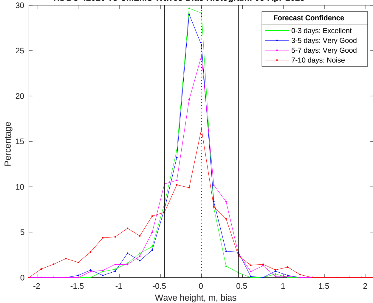
NDBC 42020 vs CMEMS Waves Bias Histogram: 08-Apr-2025
