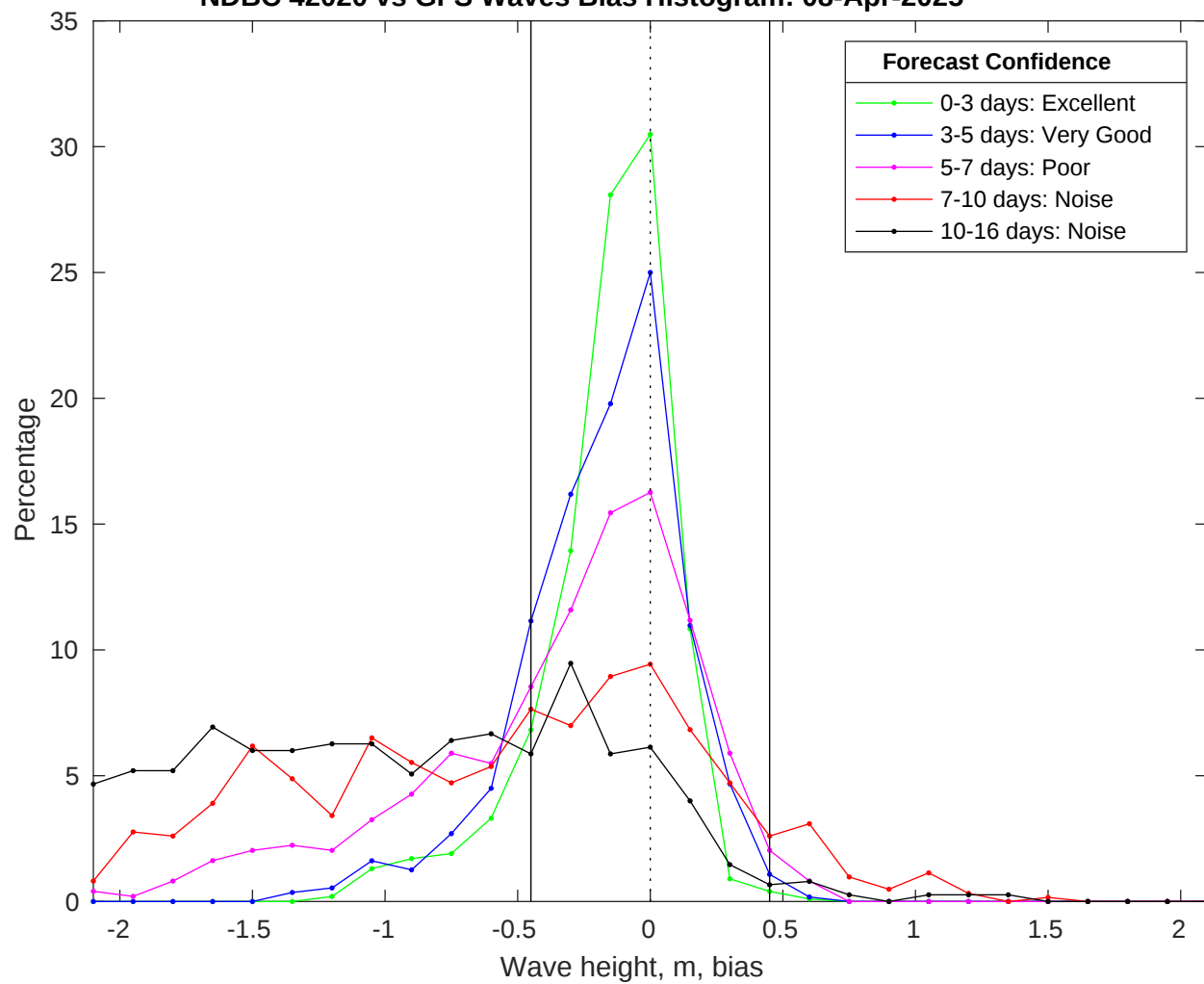
NDBC 42020 vs GFS Waves Bias Histogram: 08-Apr-2025
