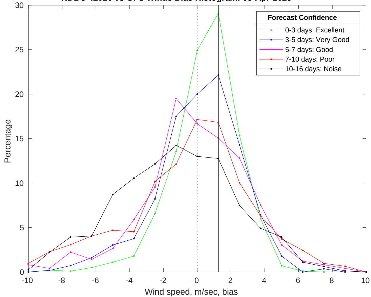
NDBC 42020 vs GFS Winds Bias Histogram: 08-Apr-2025
