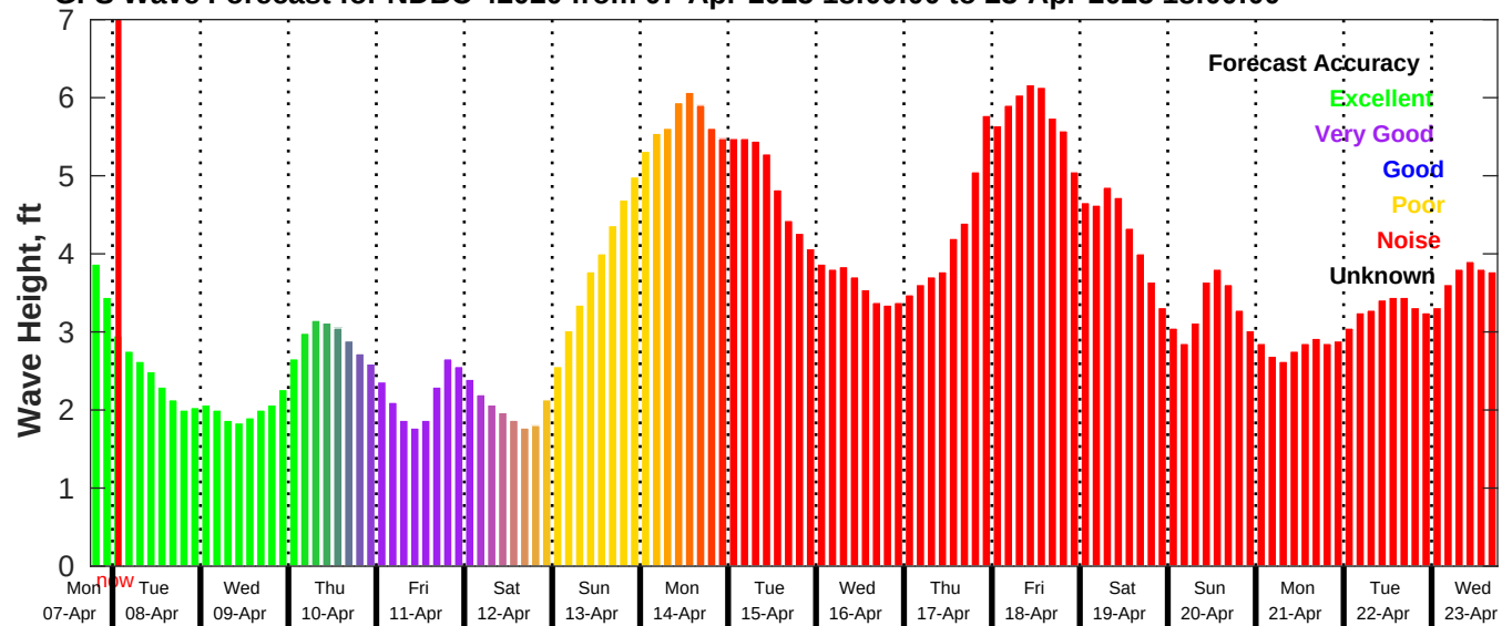
GFS Wave Forecast for NDBC 42020 from 07-Apr-2025 18:00:00 to 23-Apr-2025 18:00:00
