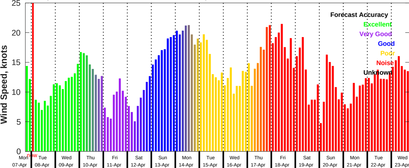
GFS Wind Speed Forecast for NDBC 42020 from 07-Apr-2025 18:00:00 to 23-Apr-2025 18:00:00
