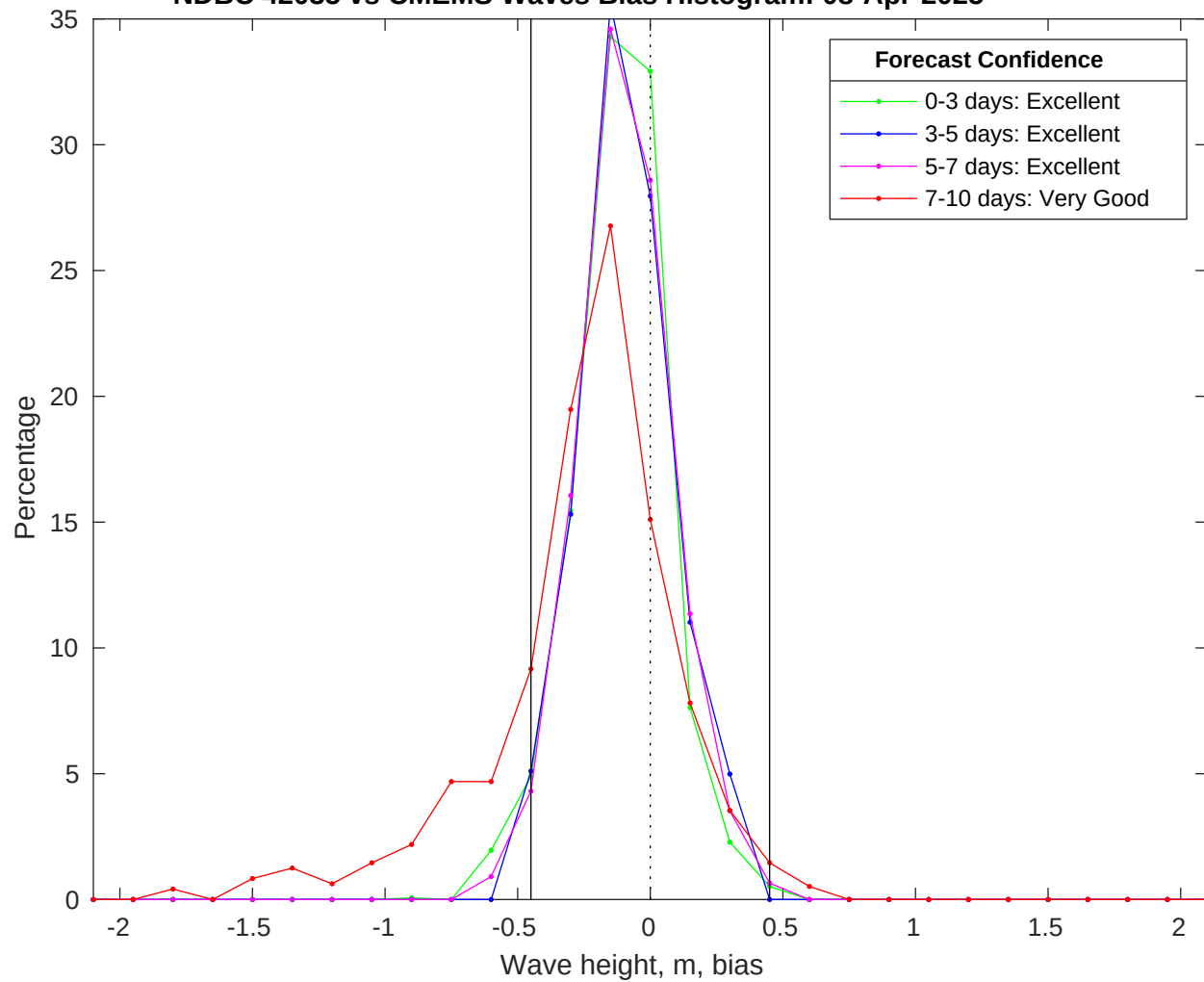
NDBC 42035 vs CMEMS Waves Bias Histogram: 08-Apr-2025
