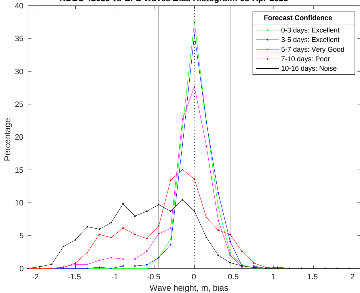
NDBC 42035 vs GFS Waves Bias Histogram: 08-Apr-2025
