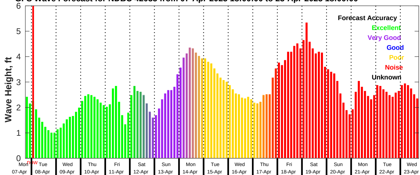
GFS Wave Forecast for NDBC 42035 from 07-Apr-2025 18:00:00 to 23-Apr-2025 18:00:00
