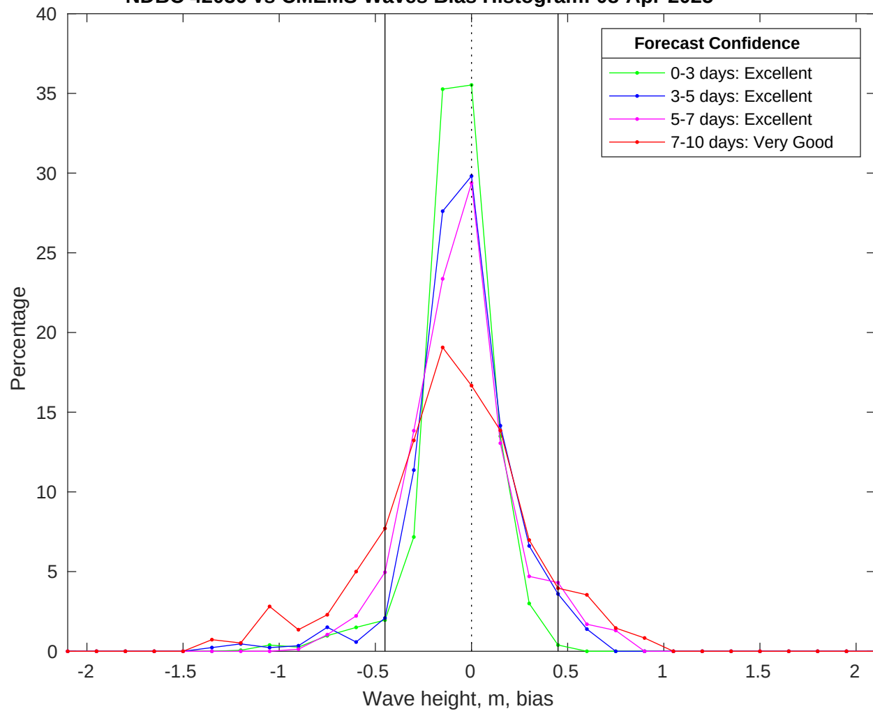
NDBC 42036 vs CMEMS Waves Bias Histogram: 08-Apr-2025
