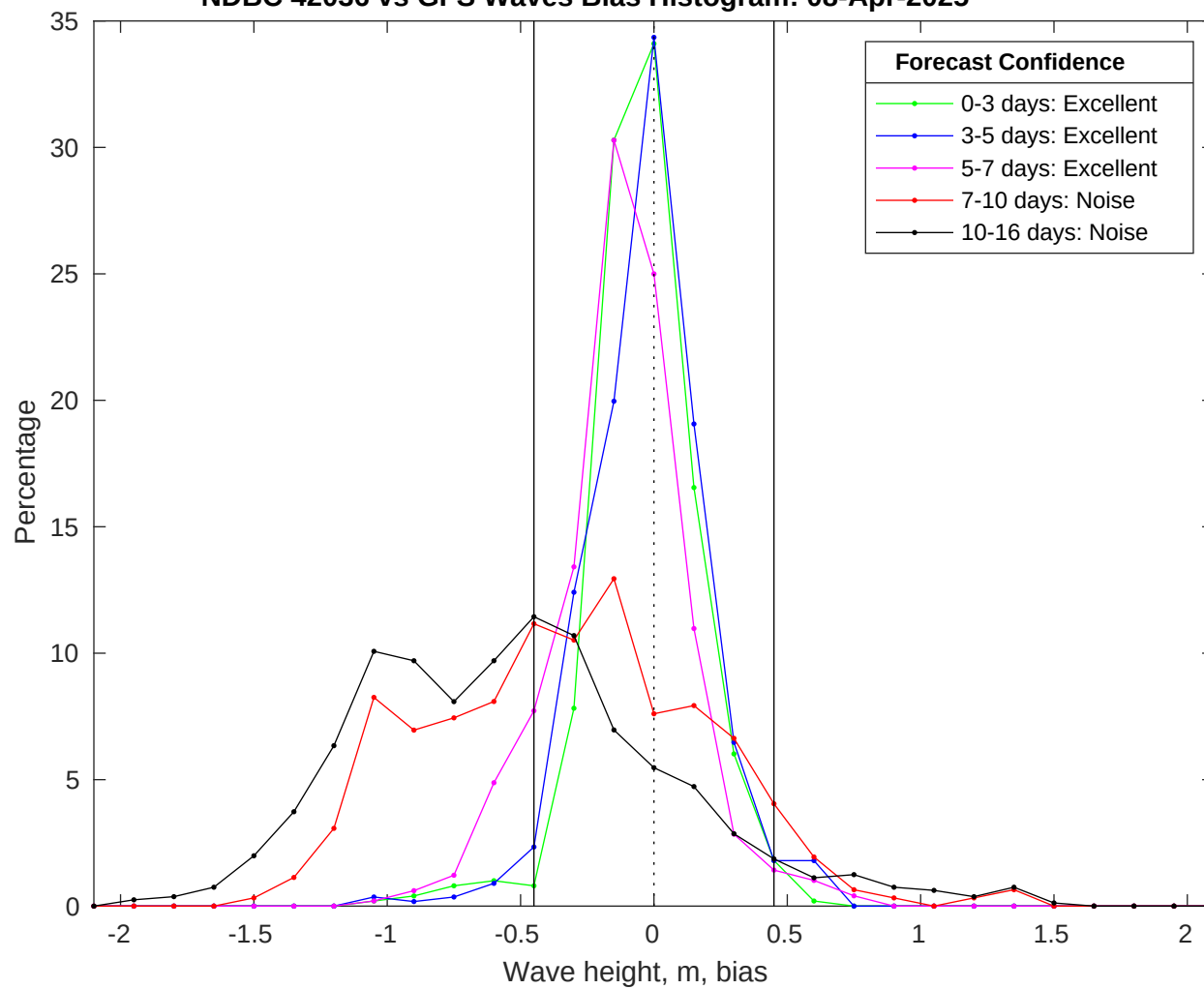
NDBC 42036 vs GFS Waves Bias Histogram: 08-Apr-2025
