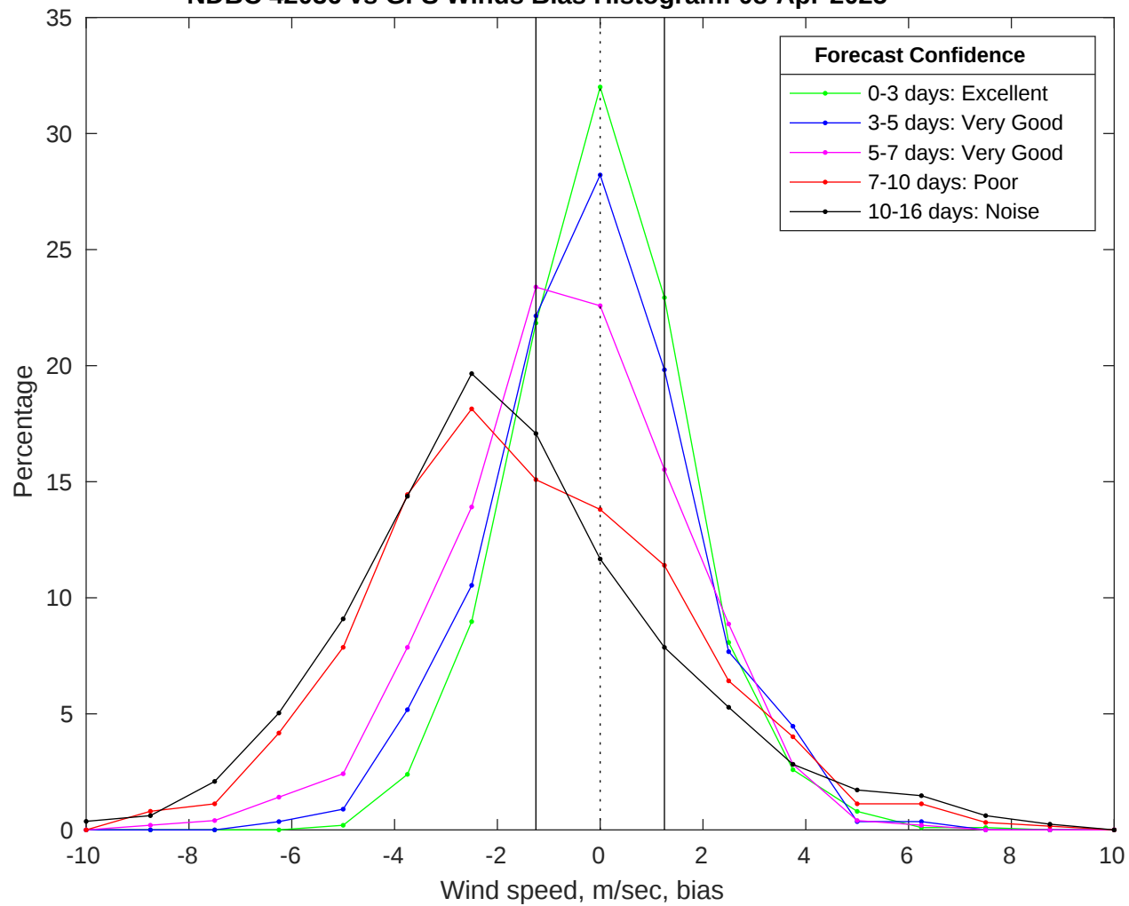
NDBC 42036 vs GFS Winds Bias Histogram: 08-Apr-2025
