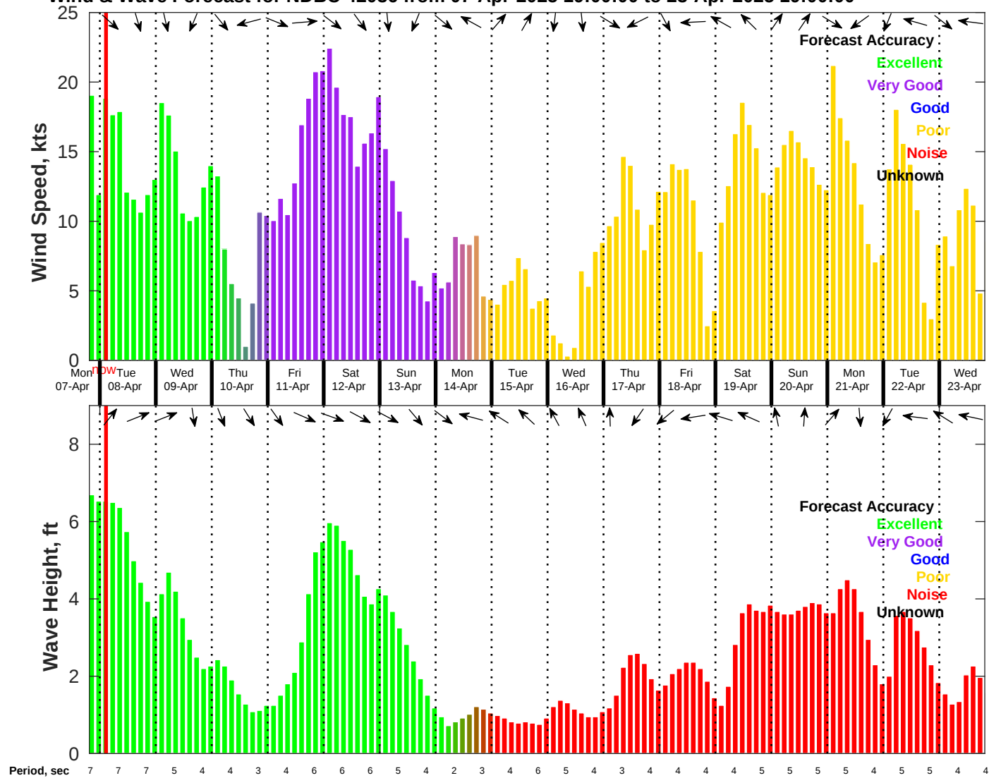
Wind & Wave Forecast for NDBC 42036 from 07-Apr-2025 19:00:00 to 23-Apr-2025 19:00:00
