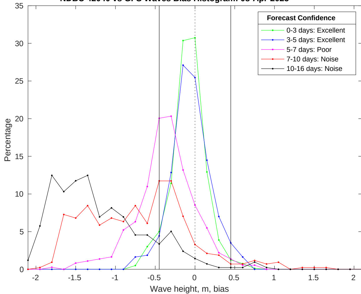
NDBC 42040 vs GFS Waves Bias Histogram: 08-Apr-2025
