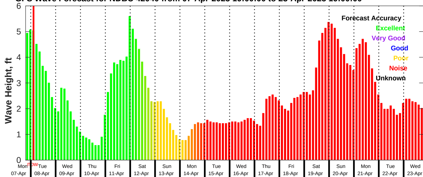
GFS Wave Forecast for NDBC 42040 from 07-Apr-2025 19:00:00 to 23-Apr-2025 19:00:00
