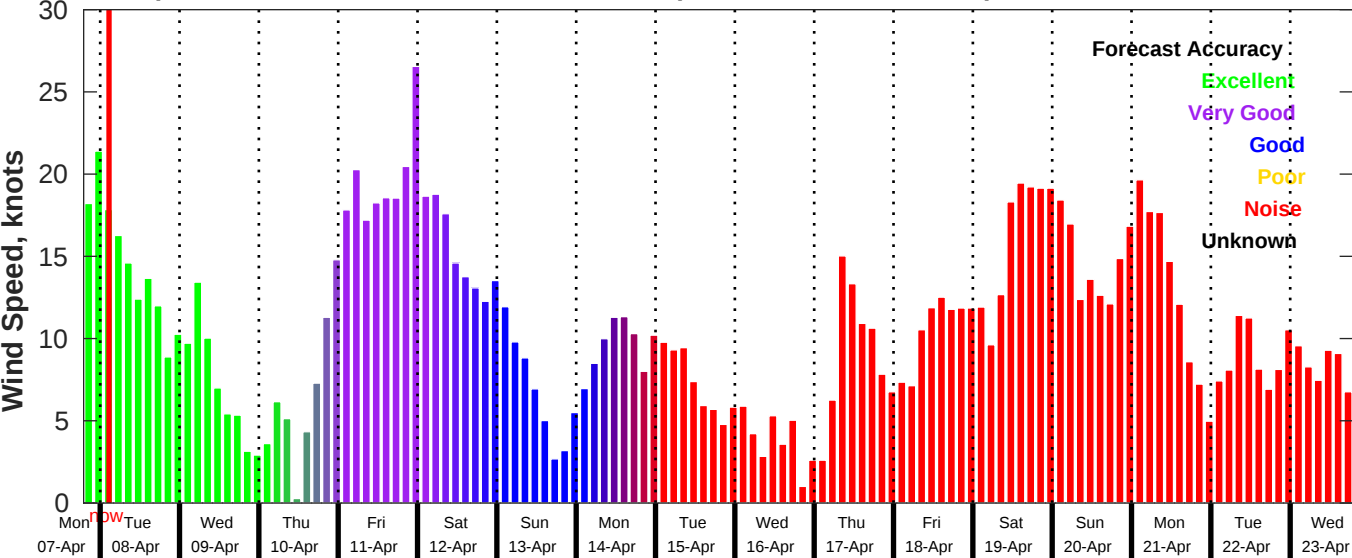
GFS Wind Speed Forecast for NDBC 42040 from 07-Apr-2025 19:00:00 to 23-Apr-2025 19:00:00
