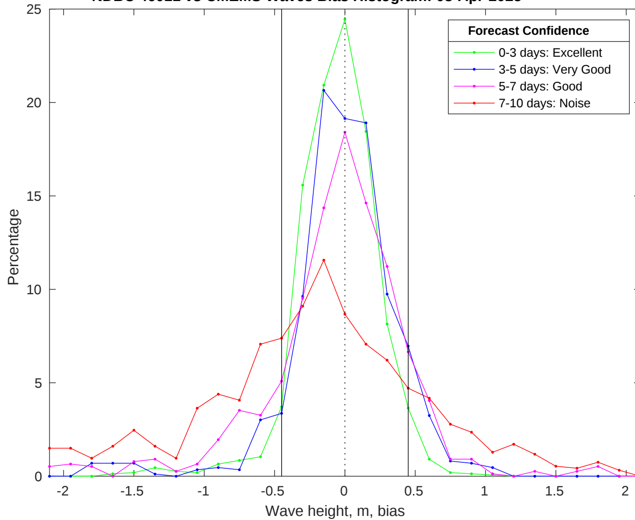
NDBC 46011 vs CMEMS Waves Bias Histogram: 08-Apr-2025
