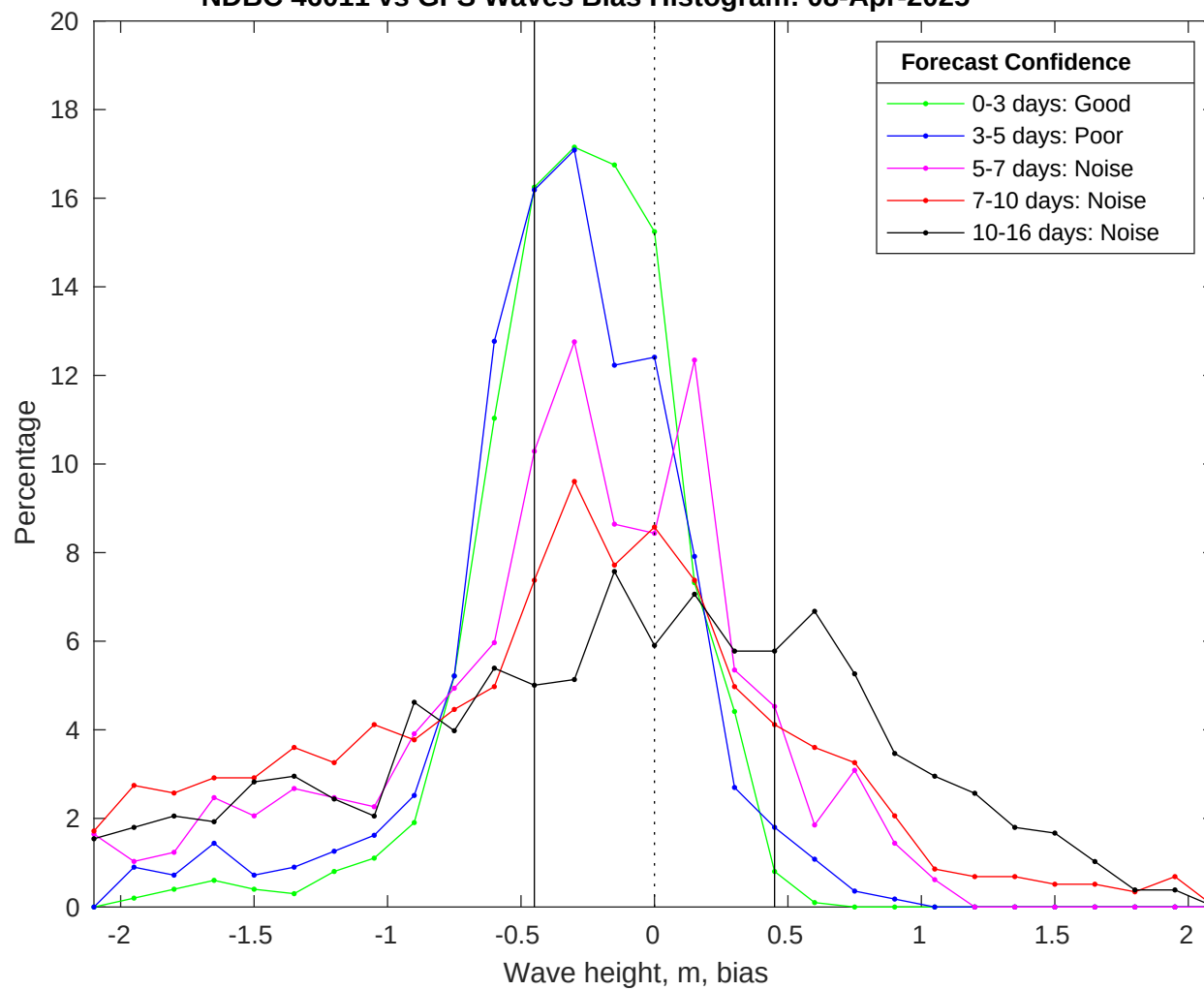
NDBC 46011 vs GFS Waves Bias Histogram: 08-Apr-2025
