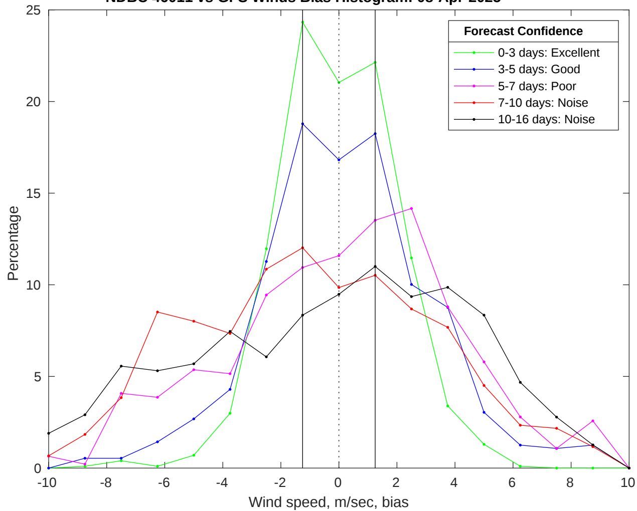
NDBC 46011 vs GFS Winds Bias Histogram: 08-Apr-2025
