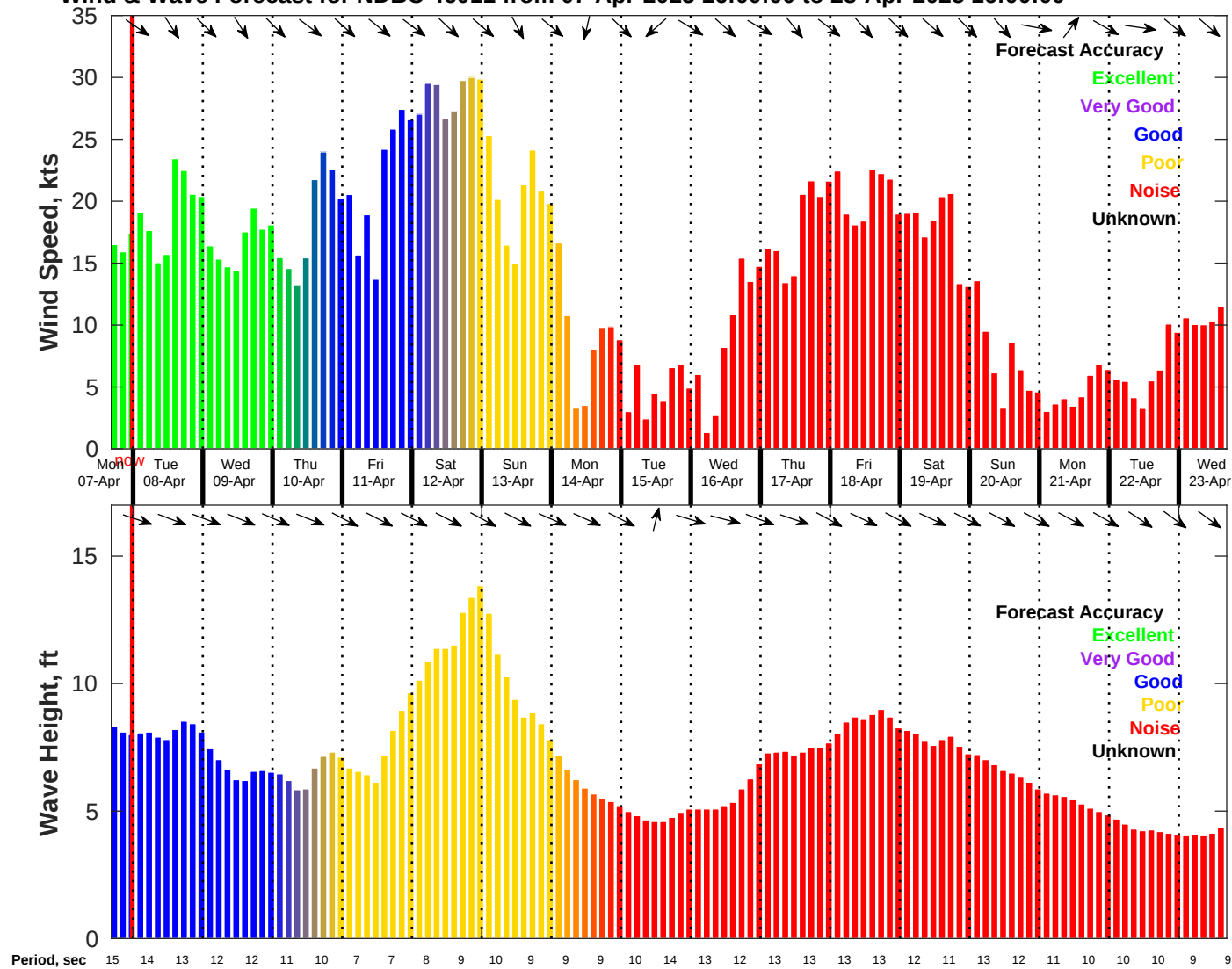
Wind & Wave Forecast for NDBC 46011 from 07-Apr-2025 16:00:00 to 23-Apr-2025 16:00:00
