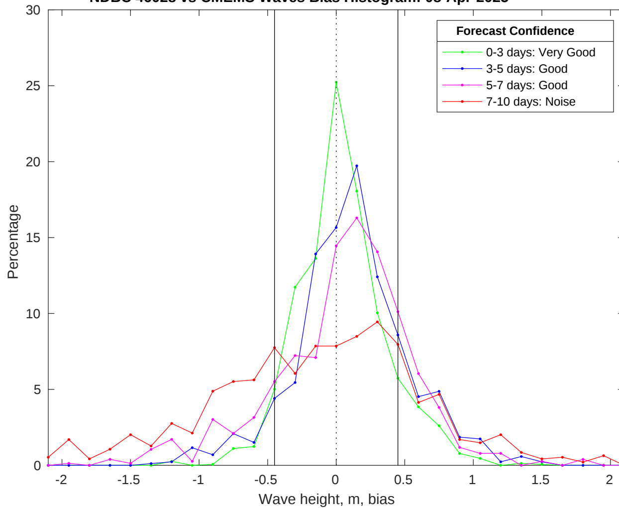
NDBC 46028 vs CMEMS Waves Bias Histogram: 08-Apr-2025
