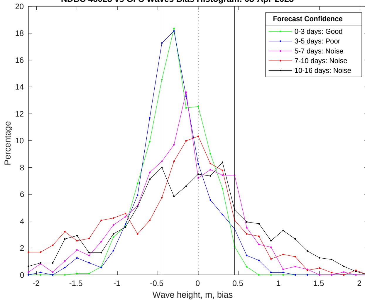
NDBC 46028 vs GFS Waves Bias Histogram: 08-Apr-2025
