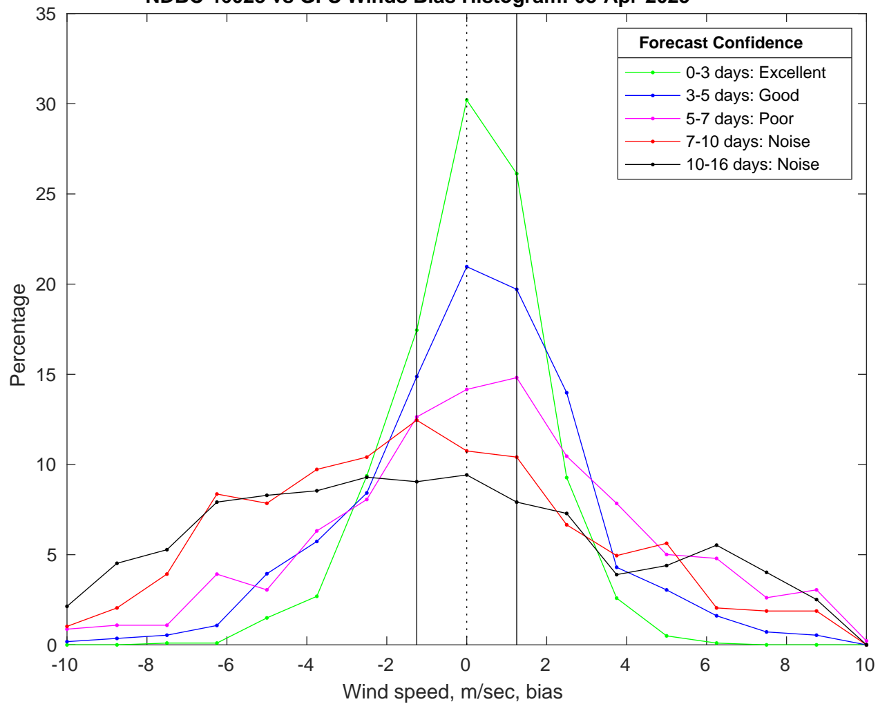
NDBC 46028 vs GFS Winds Bias Histogram: 08-Apr-2025
