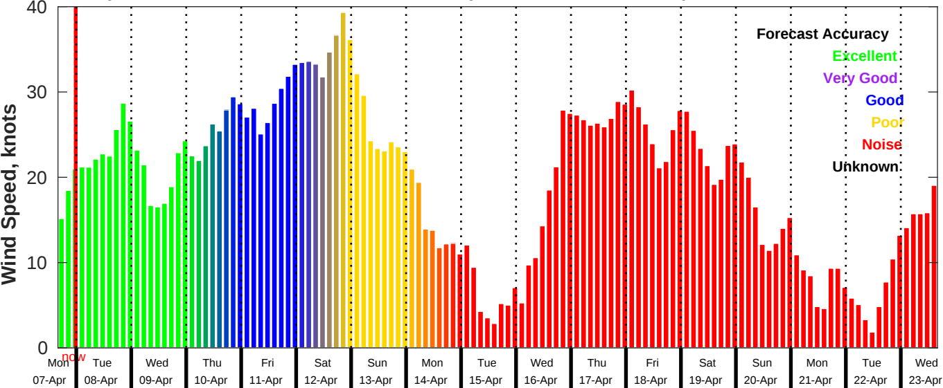
GFS Wind Speed Forecast for NDBC 46028 from 07-Apr-2025 16:00:00 to 23-Apr-2025 16:00:00
