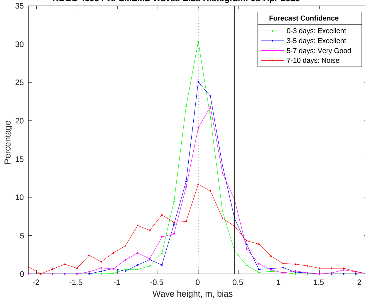
NDBC 46054 vs CMEMS Waves Bias Histogram: 08-Apr-2025
