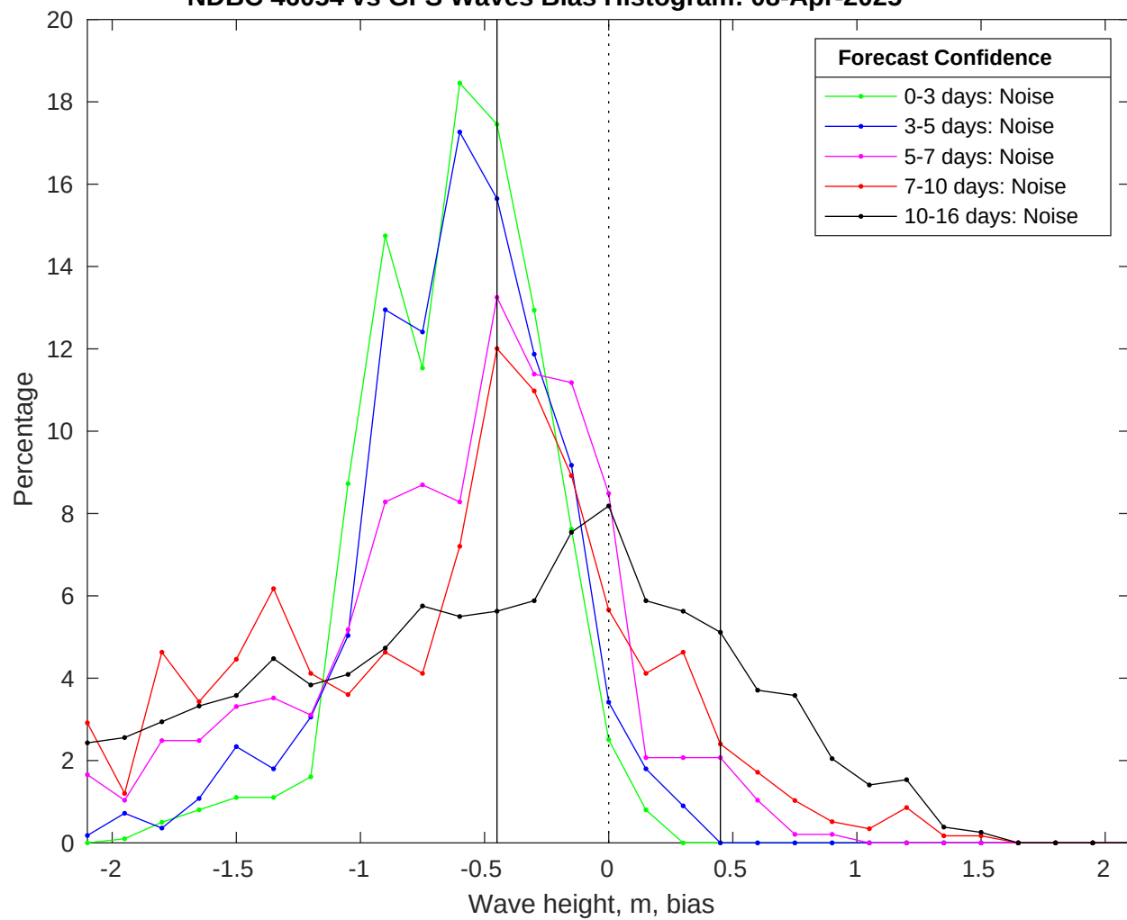
NDBC 46054 vs GFS Waves Bias Histogram: 08-Apr-2025
