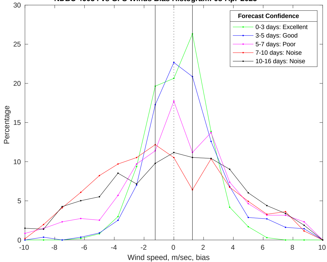
NDBC 46054 vs GFS Winds Bias Histogram: 08-Apr-2025
