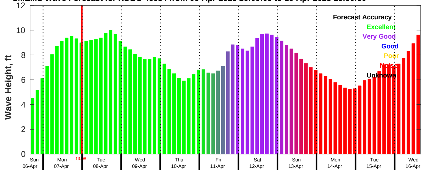
CMEMS Wave Forecast for NDBC 46054 from 06-Apr-2025 16:00:00 to 16-Apr-2025 16:00:00
