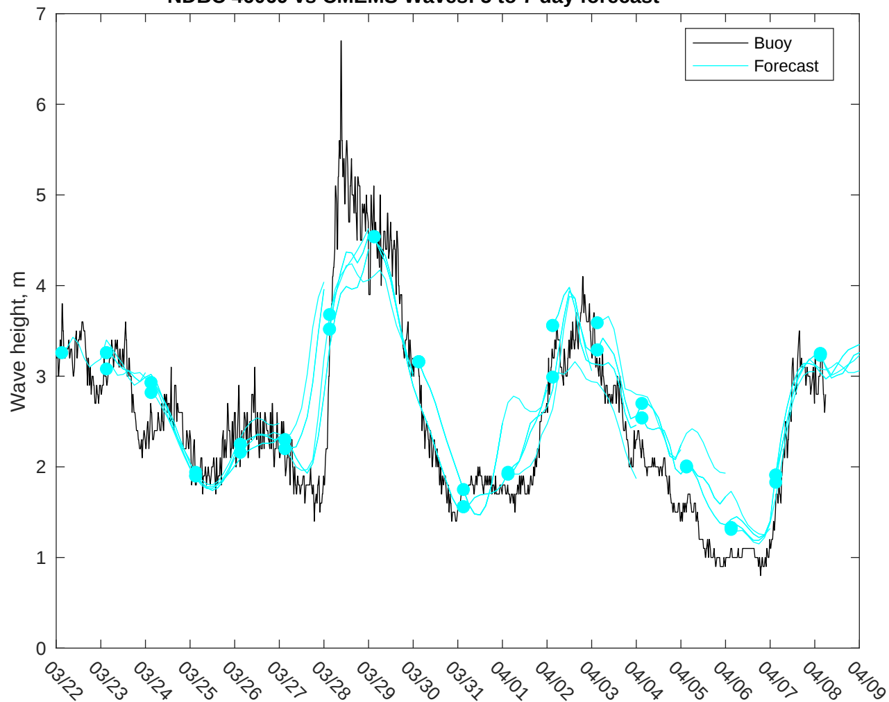
NDBC 46069 vs CMEMS Waves: 5 to 7 day forecast
