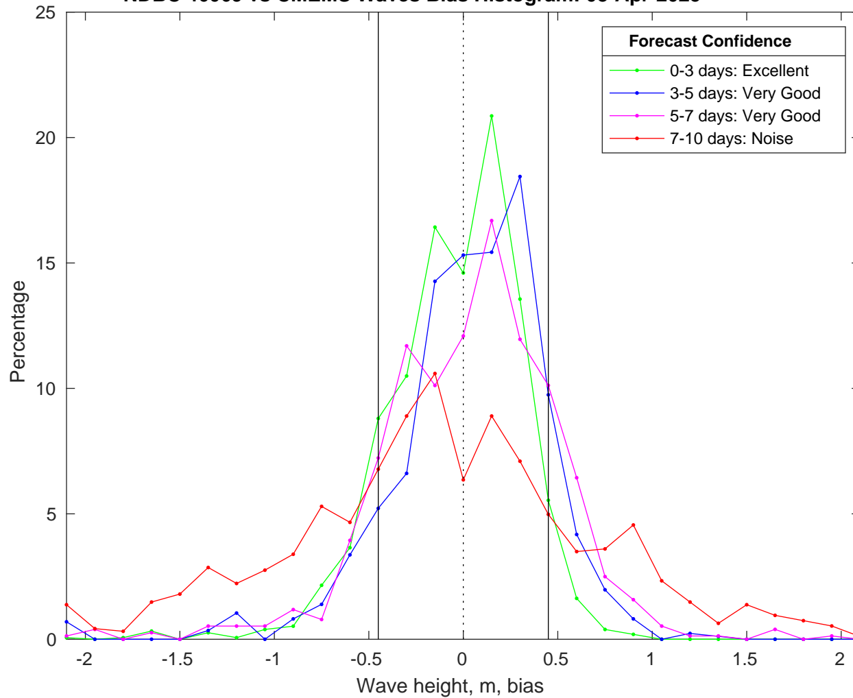
NDBC 46069 vs CMEMS Waves Bias Histogram: 08-Apr-2025
