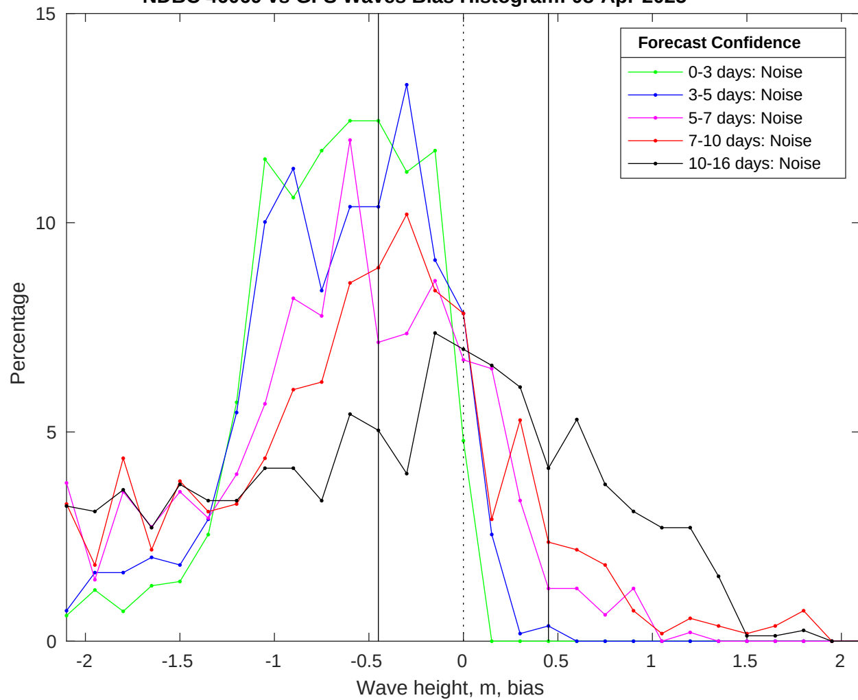
NDBC 46069 vs GFS Waves Bias Histogram: 08-Apr-2025
