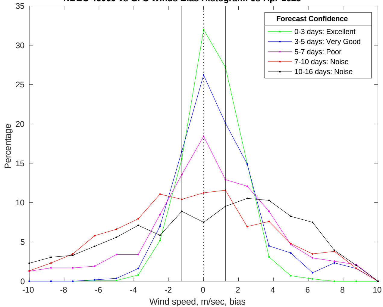
NDBC 46069 vs GFS Winds Bias Histogram: 08-Apr-2025
