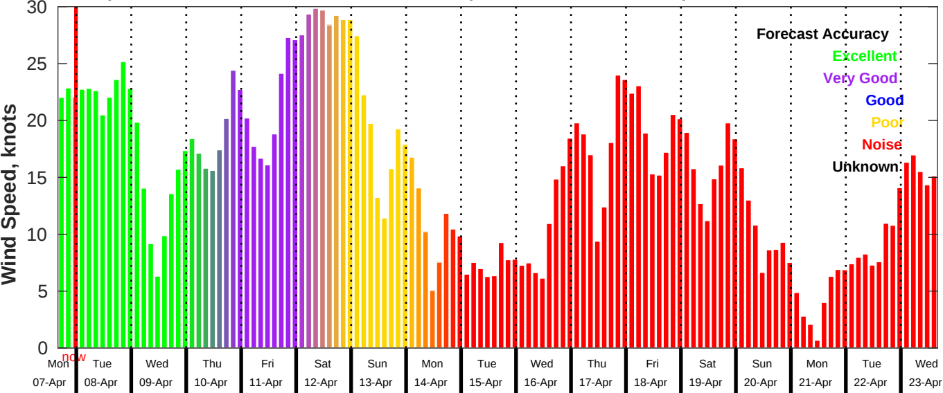
GFS Wind Speed Forecast for NDBC 46069 from 07-Apr-2025 16:00:00 to 23-Apr-2025 16:00:00
