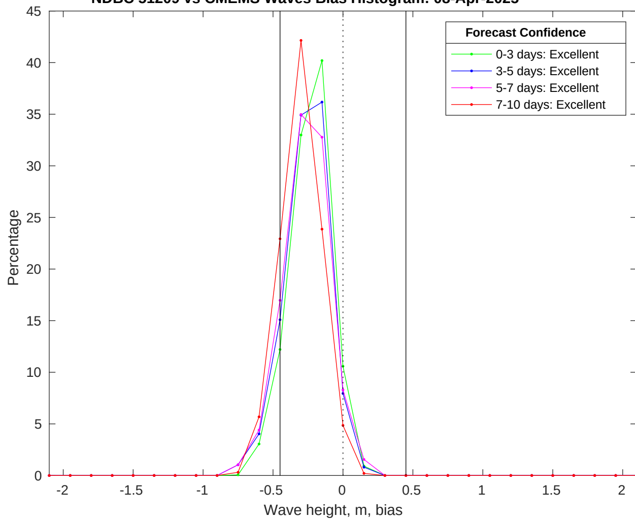
NDBC 51209 vs CMEMS Waves Bias Histogram: 08-Apr-2025
