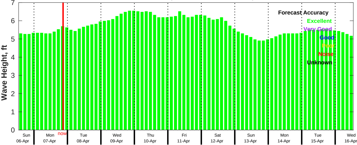
CMEMS Wave Forecast for NDBC 51209 from 06-Apr-2025 13:00:00 to 16-Apr-2025 13:00:00
