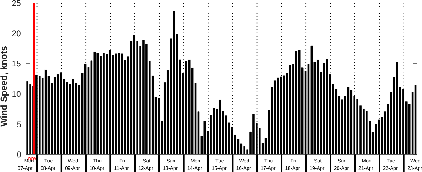
GFS Wind Speed Forecast for NDBC 51209 from 07-Apr-2025 13:00:00 to 23-Apr-2025 13:00:00
