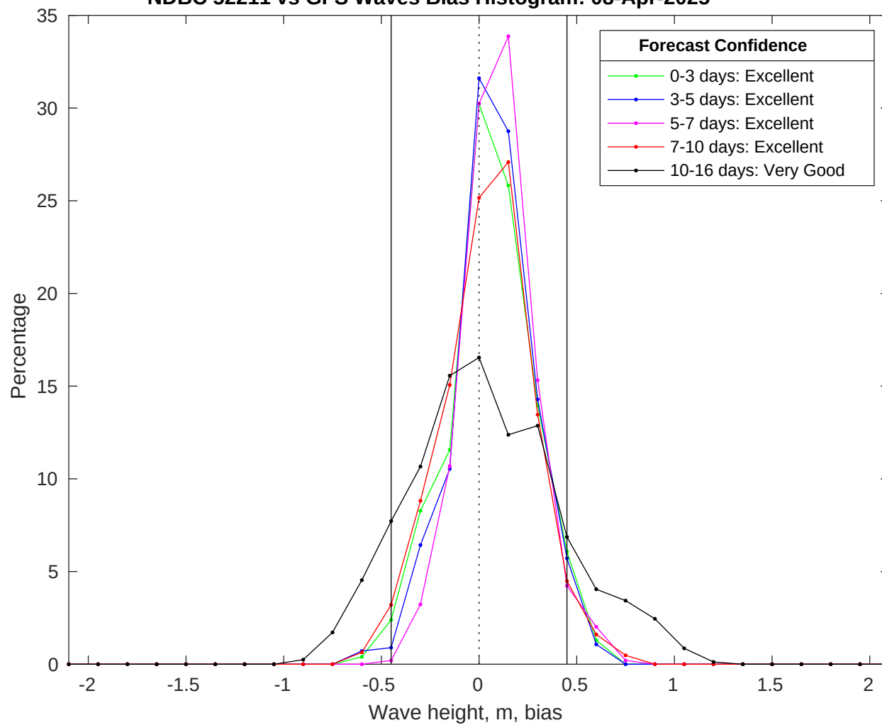
NDBC 52211 vs GFS Waves Bias Histogram: 08-Apr-2025
