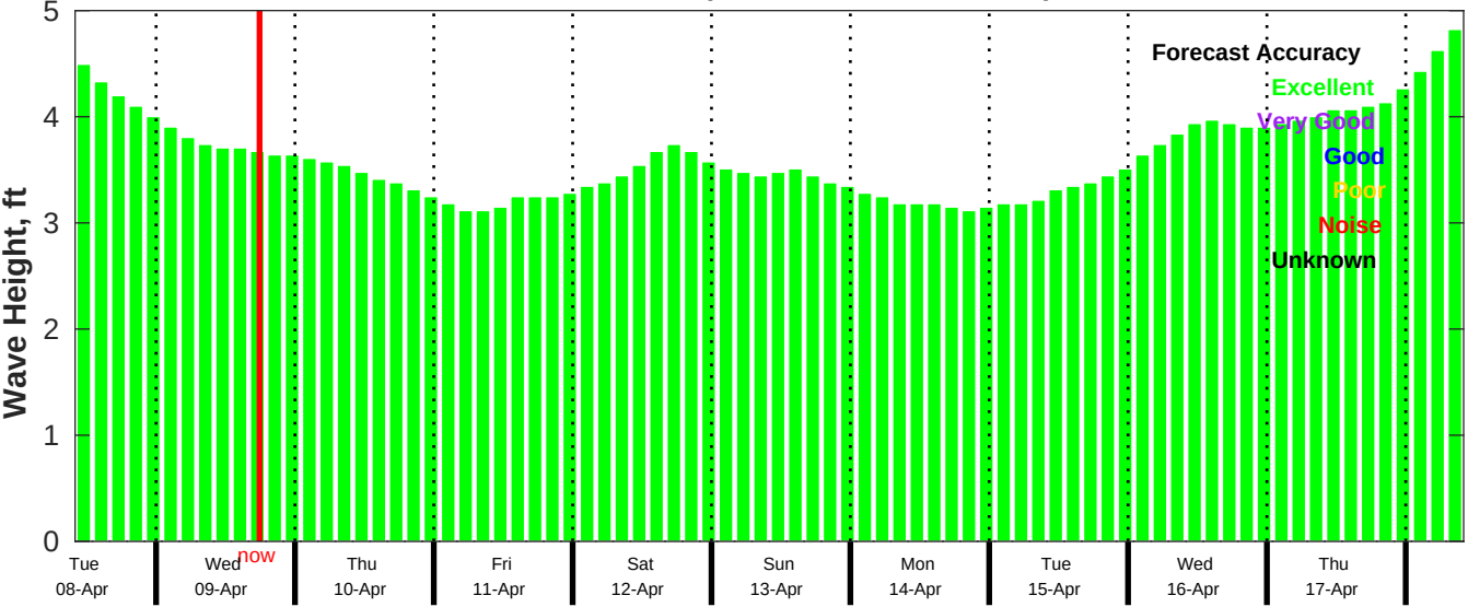
CMEMS Wave Forecast for NDBC 52211 from 07-Apr-2025 10:00:00 to 17-Apr-2025 10:00:00
