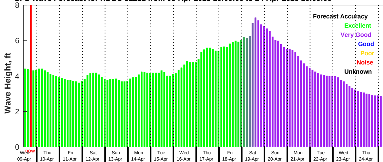
GFS Wave Forecast for NDBC 52211 from 08-Apr-2025 10:00:00 to 24-Apr-2025 10:00:00
