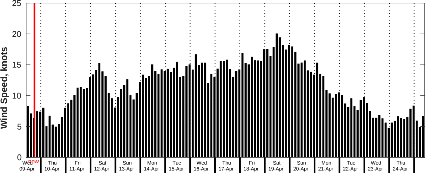
GFS Wind Speed Forecast for NDBC 52211 from 08-Apr-2025 10:00:00 to 24-Apr-2025 10:00:00
