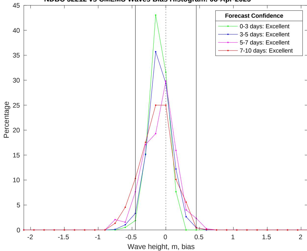
NDBC 52212 vs CMEMS Waves Bias Histogram: 08-Apr-2025
