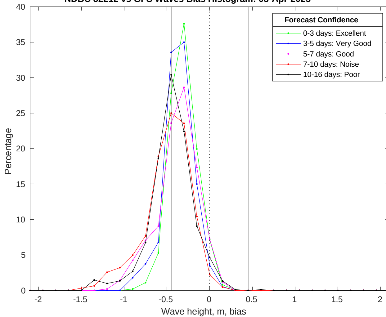
NDBC 52212 vs GFS Waves Bias Histogram: 08-Apr-2025
