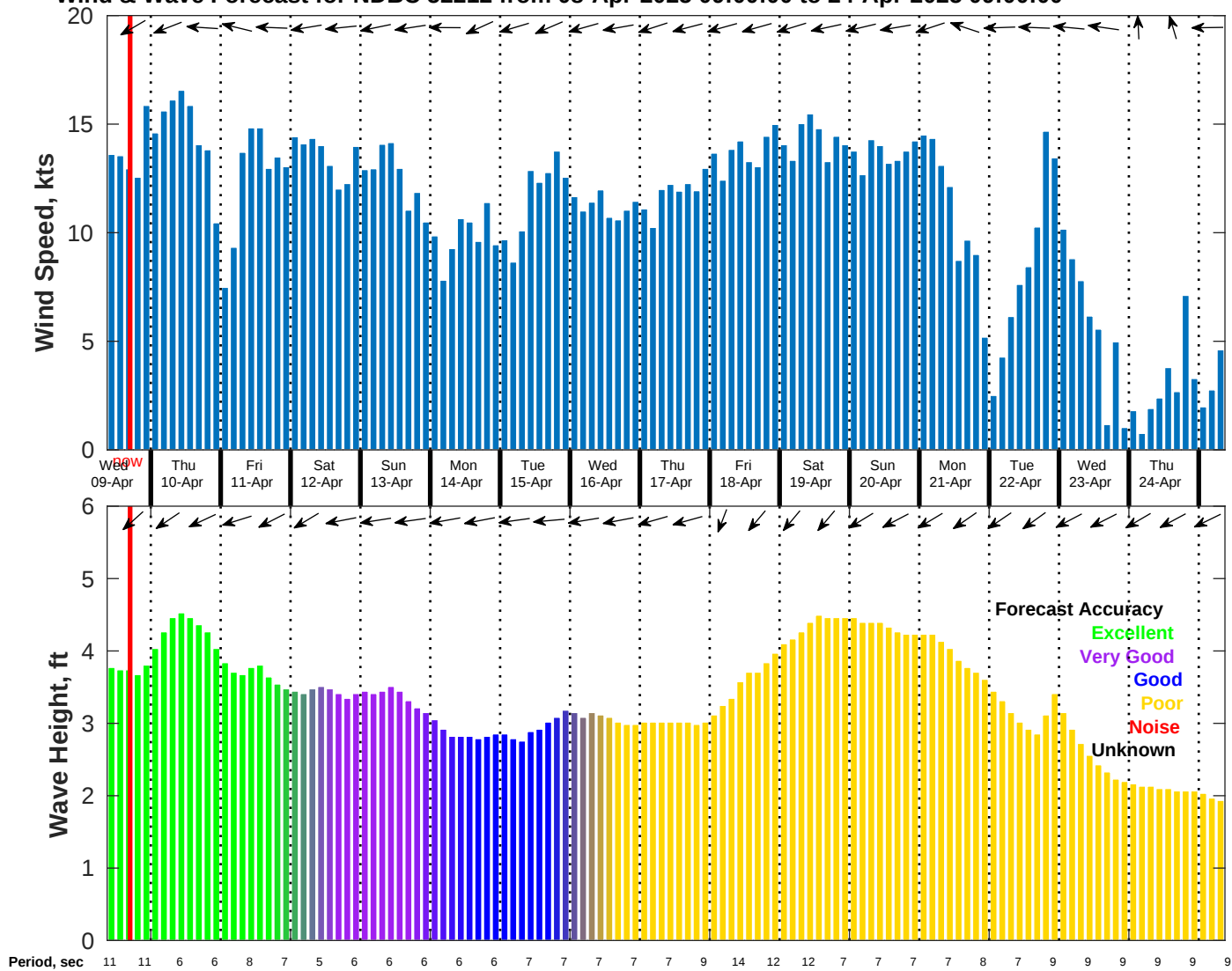
Wind & Wave Forecast for NDBC 52212 from 08-Apr-2025 09:00:00 to 24-Apr-2025 09:00:00
